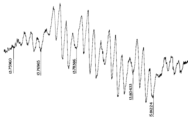
Figure 2. Low-field multiplet for \text{Me}_3\text{C}\dot{N}CO^{13}\text{CH}_3 at 195 K showing a^{13C} = 4.6 G, a^H(3\text{ H}) = 2.45 G, and a^H(9\text{ H}) = 0.56 G. Field markers are given in MHz (uncorrected). The average microwave frequency was 9133.80 MHz.
