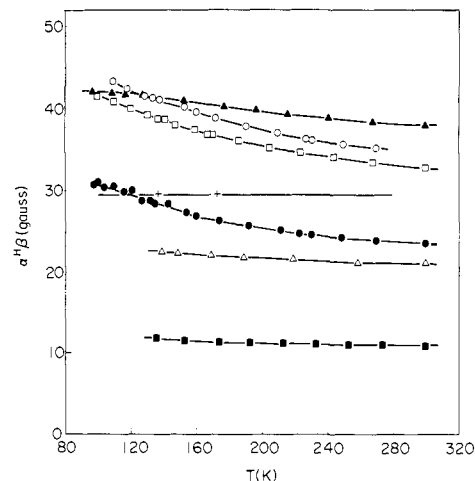
Figure 1. Values of a^{H\beta} as a function of temperature for t -BuCH 2 NCO- t -Bu, \blacktriangle ; EtNCOEt, \circ ; EtNCO- t -Bu, \square ; MeNCOEt, + ; i -PrNCOEt, \bullet ; i -PrNCO- t -Bu, \triangle ; t -Bu 2 CHNCOME, \blacksquare .
